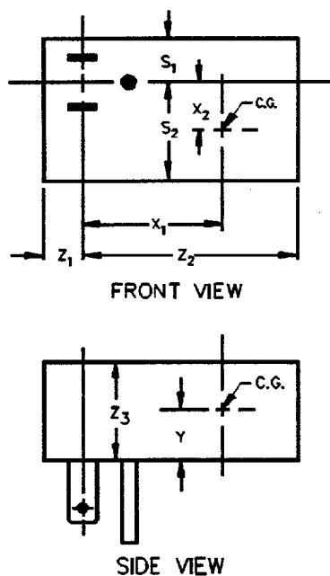
Figure 10.1 Dimensions of a direct plug-in unit
