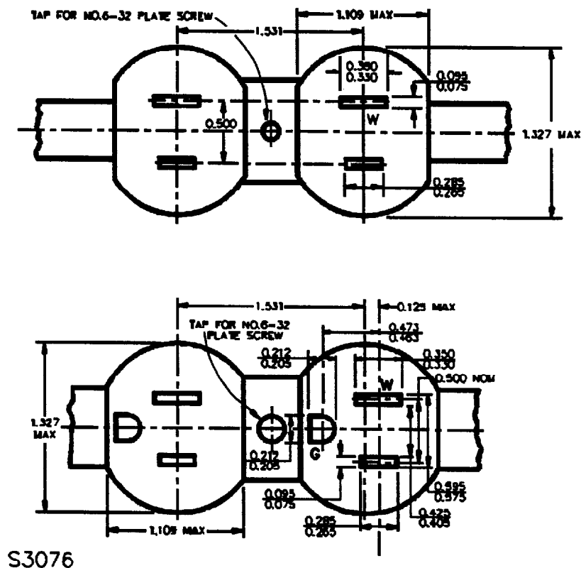
Figure 10.2 Parallel duplex receptacle
