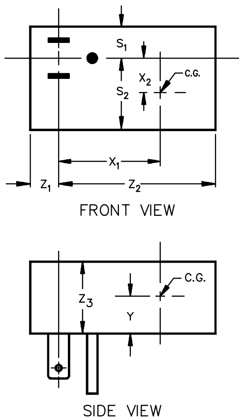
Figure 6.1 Dimensions of a direct plug-in unit
