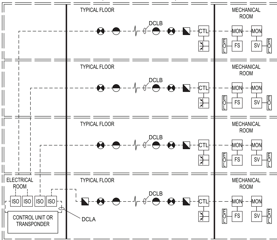
FIGURE 2.6 FLOOR DATA COMMUNICATION LINK B (DCLB) CIRCUITS CONNECTED TO DATA COMMUNICATION LINK A (DCLA) INSTALLED IN A SINGLE FIRE-RATED ELECTRICAL ROOM
