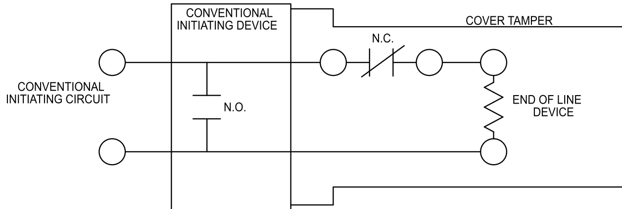
FIGURE 31.1 EXAMPLE OF TAMPER DEVICE SERVING FIRE SUPPRESSION SYSTEM
