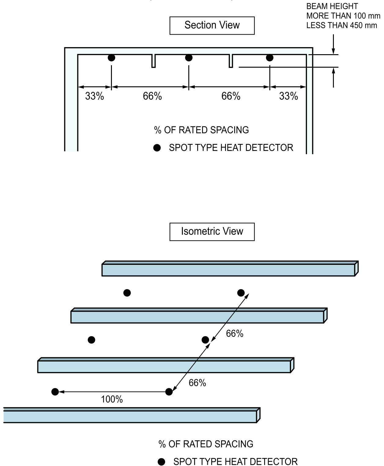
FIGURE 21 SPACING OF SPOT TYPE HEAT DETECTORS FOR BEAM CONSTRUCTION
