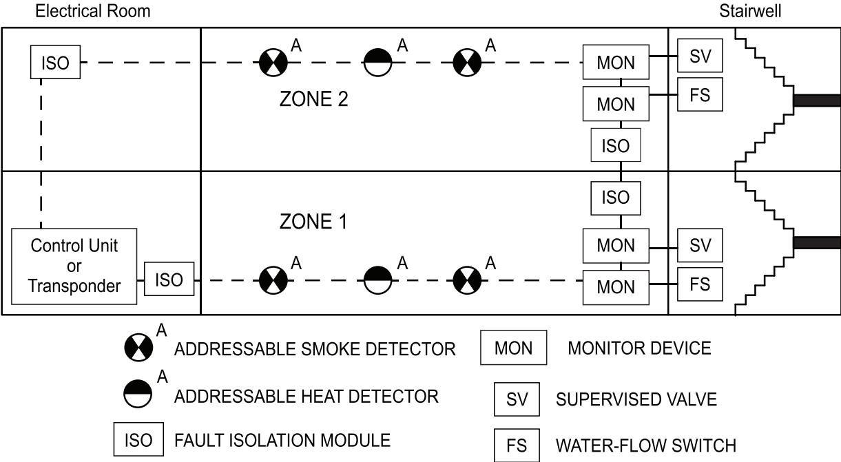
FIGURE 31.2 EXAMPLE OF SUPPORTING FIELD DEVICES SERVING FIRE SUPPRESSION SYSTEM (Reference: Clause 12.3.13)
