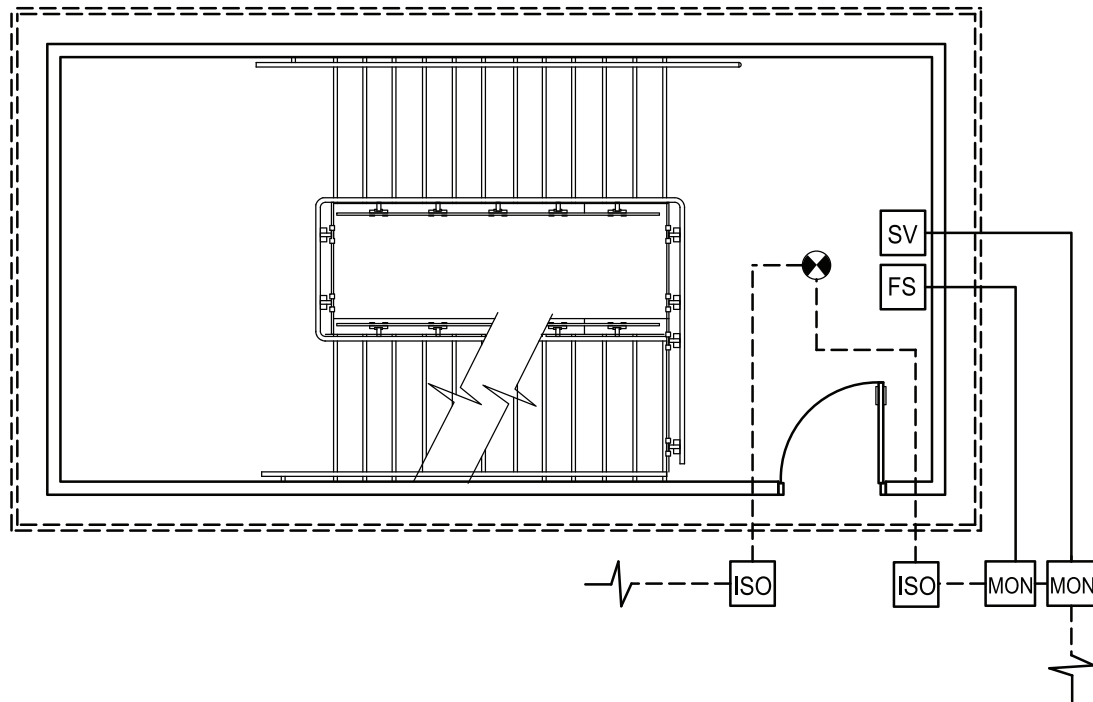
FIGURE 2.4 EXAMPLE OF FAULT ISOLATOR SERVING A SINGLE FIELD DEVICE IN AN EXIT STAIR
