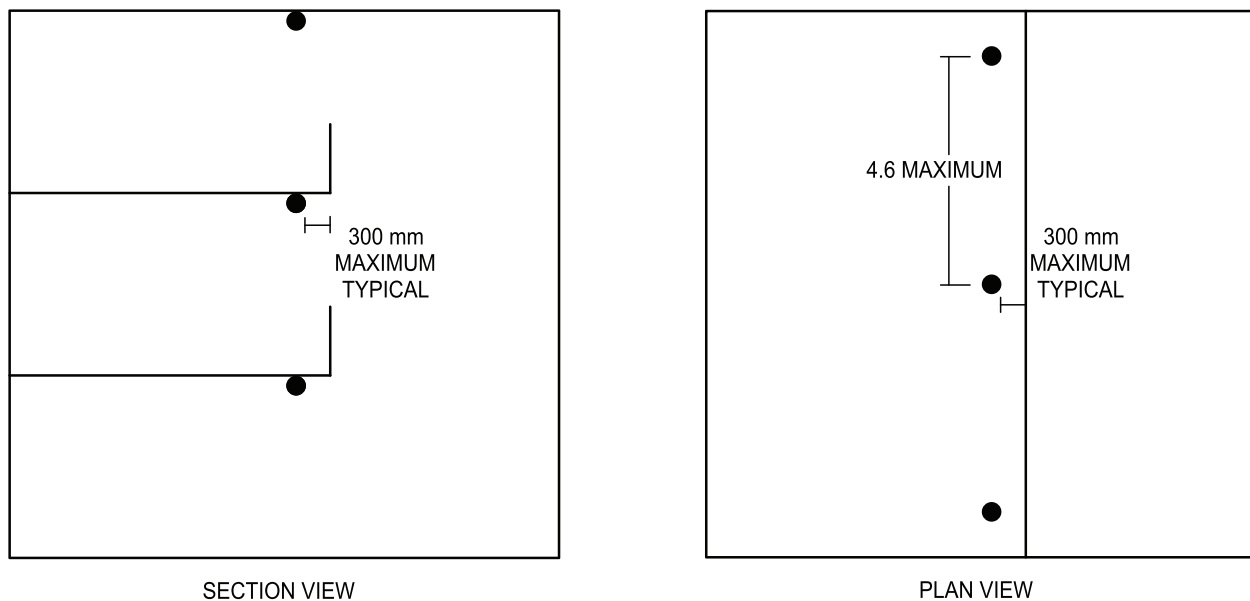
FIGURE 18.1 DETECTOR SPACING OF SMOKE DETECTORS: GALLERIES, MEZZANINE AND INTERIOR BALCONIES
