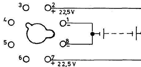
Figure 3. Wiring diagram
