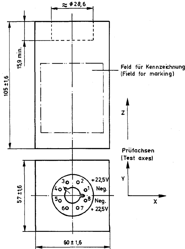
Figure 1. Dimensions
