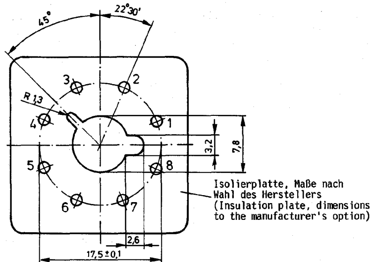
Figure 2. Plug-in connector
