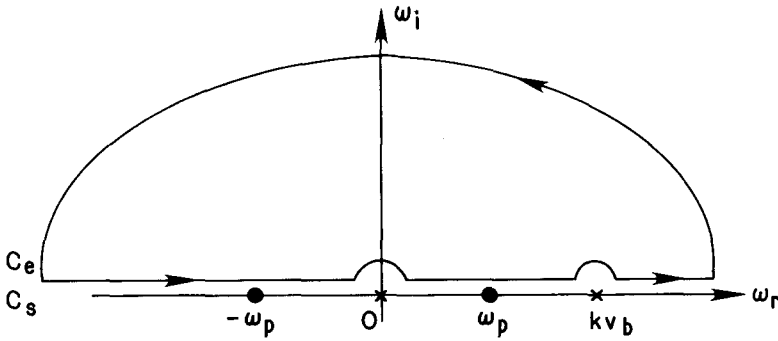
Fig. (I.5.4) \omega -plane contour for the Nyquist analysis of the beam-plasma instability dispersion relation of Eq. (I.4.15) in the kv_b > \omega_p limit.
