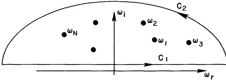
Fig. (1.5.1) Integration contour in the complex \omega plane for the Nyquist stability analysis.
