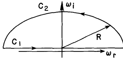
Fig. (I.5.6) w -plane contour for the Nyquist analysis of the "dispersion relation" of Eq. (I.5.11).
