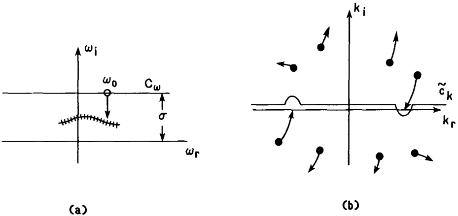
Fig. (I.6.3) Deformed contours for analytic continuations in (a) the w plane and (b) the k plane.
